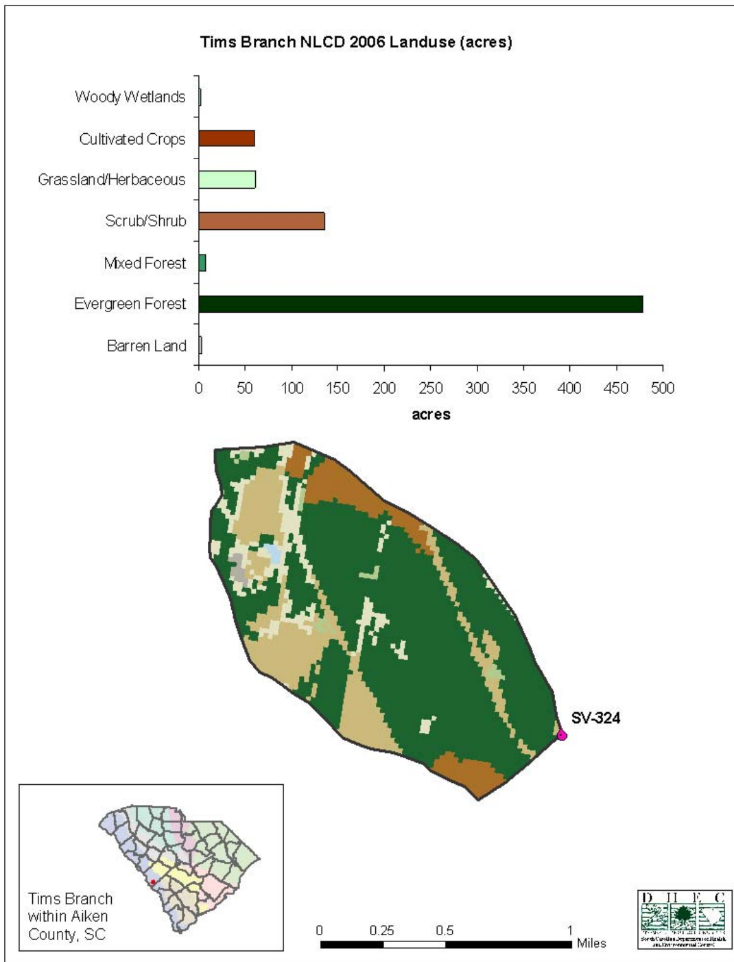
Figure 4. NLCD 2006 landuse for station SV-324, Tims Branch.
