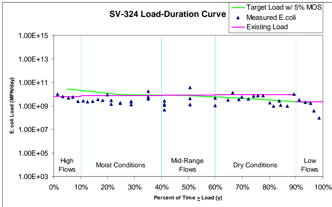
Figure 11. Load Duration Curve for station SV-324.
